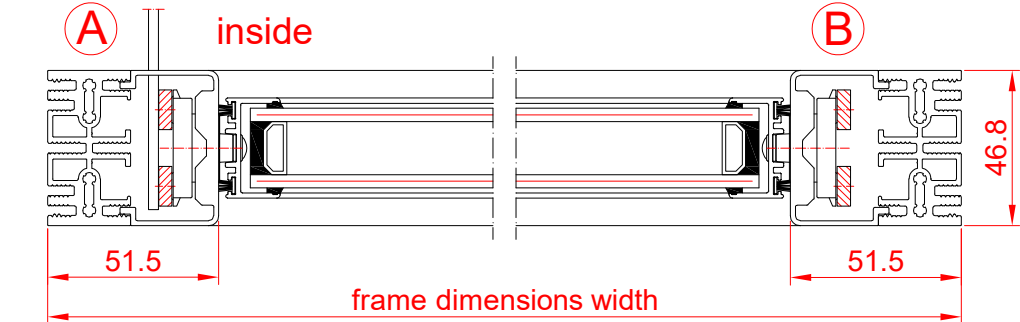
Frame type 3
