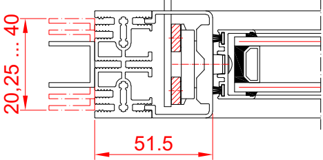
Frame type 3
