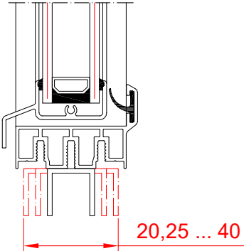
Frame type 3
