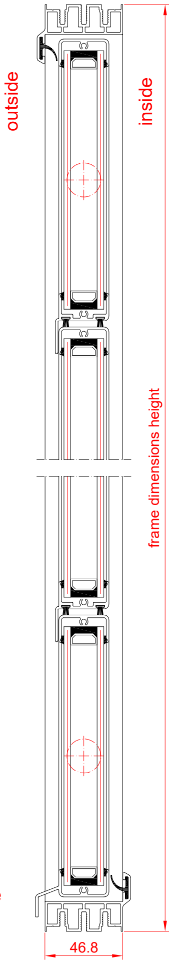
Frame type 1
