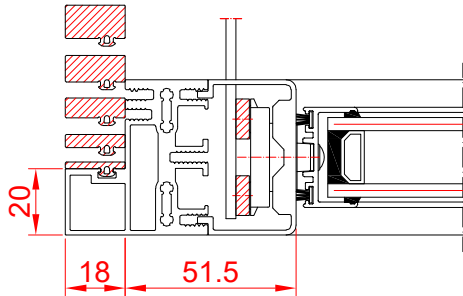
Frame type 2
