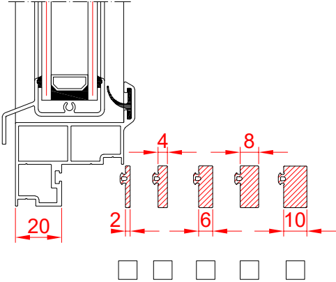
Frame type 2
