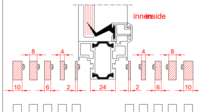
Detail frame type 2
