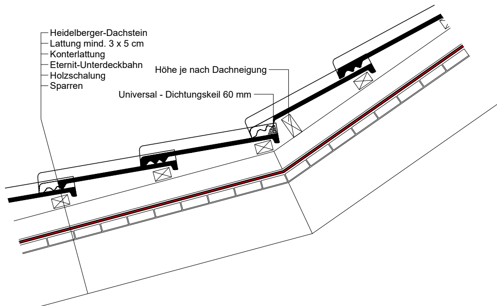
Dachknick
