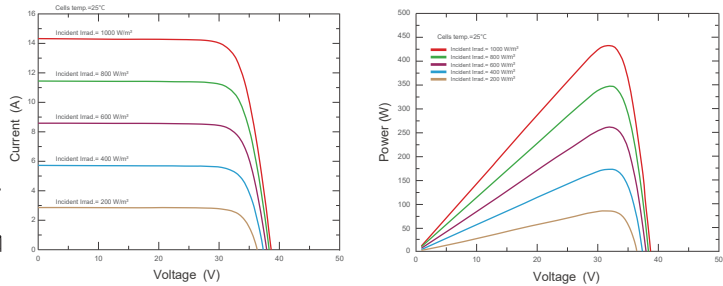
Current-Voltage & Power-Voltage Curves (FRISOLAR430M10-108D4)
