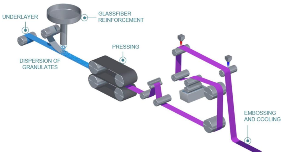
Figure 5: Pressing process diagram
