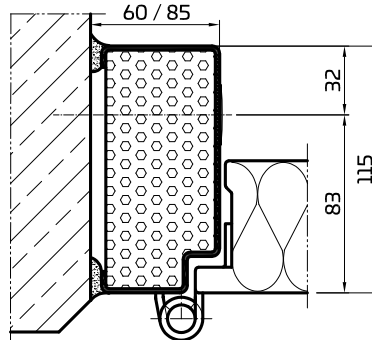
Block 60/85 00/30
