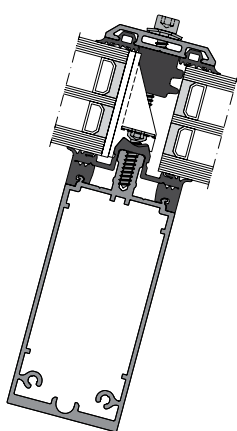
THERM + 50/56 A-I
