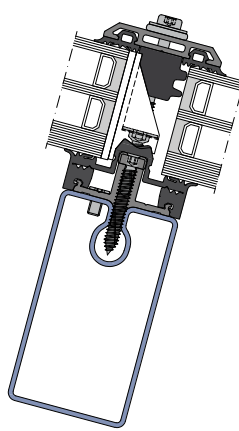
THERM + 50/56 FS-I
