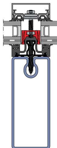
THERM + 50/56 FS-I
