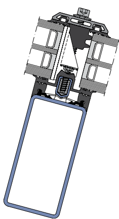
THERM + 50/56/76/96 S-I
