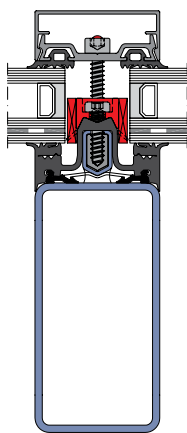
THERM + 50/56/76 S-I
