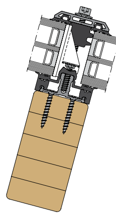
THERM + 50/56/76/96 H-I
