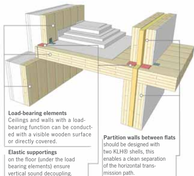
BUILDING PARTS VISIBLE CEILING
